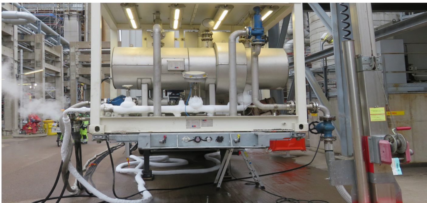
Linde's high flow nitrogen vaporizer in action, delivering 6 000 Nm 3 /h nitrogen at 6 bar g and +5 °C, for reactor cooling at a refinery.
